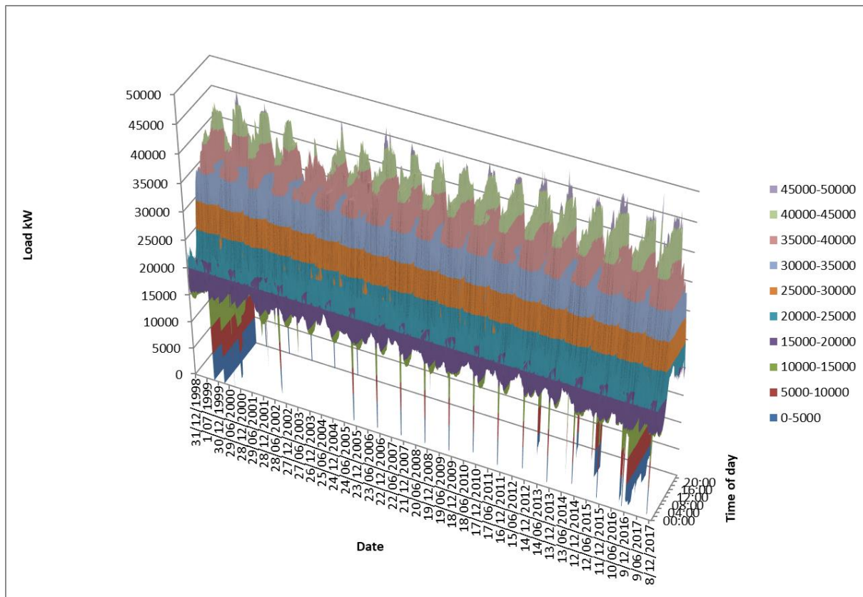
Wairoa System Historical Load 2001 to 2017
