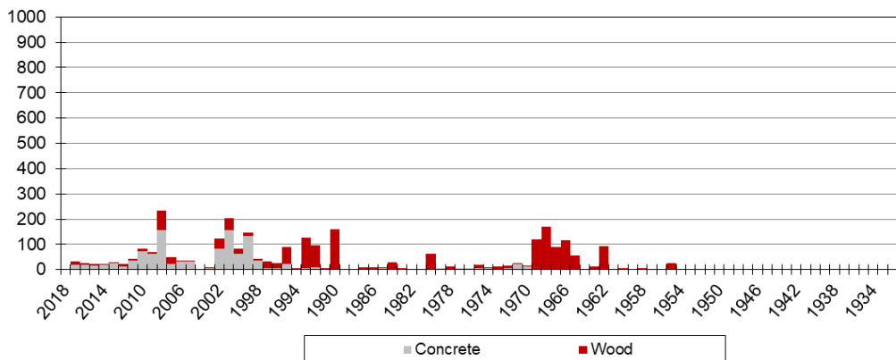
Age Profile LV Poles Urban
